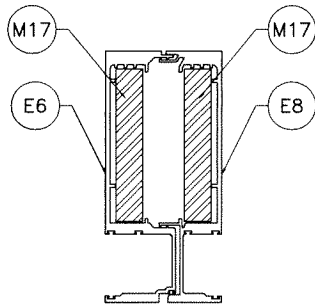
MULLION 'M3'
