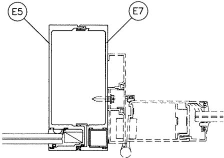
MULLION 'MD1'
